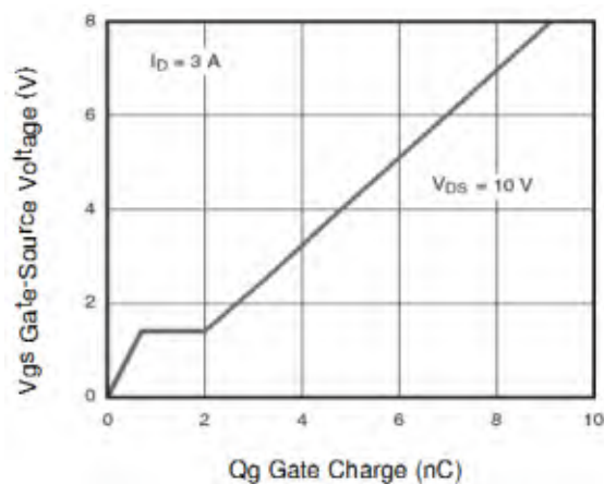
Figure 11 Gate Charge
