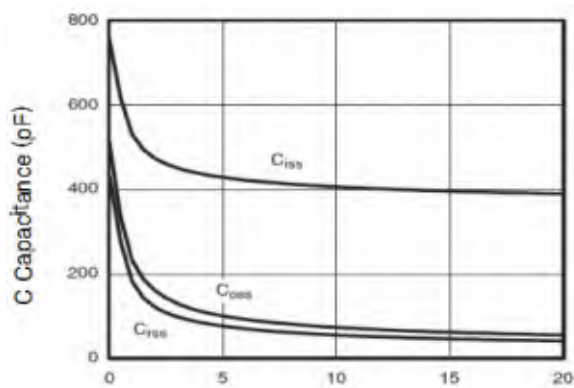
Figure 10 Capacitance vs Vds
