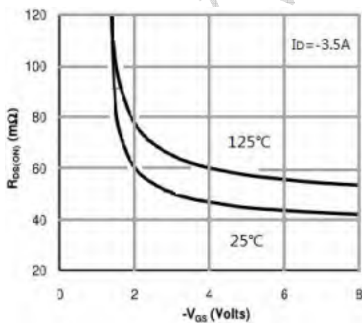
Figure 5: On-Resistance vs. Gate-Source Voltage (Note D)
