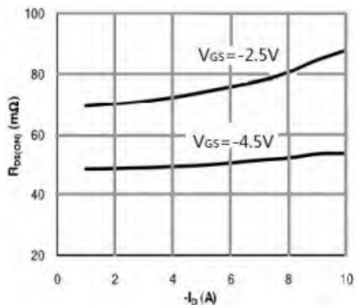
Figure 3: On-Resistance vs. Drain Current and Gate Voltage (Note D)(Note D)
