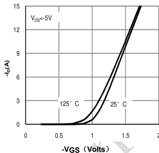
Figure 2: Transfer Characteristics (Note D)
