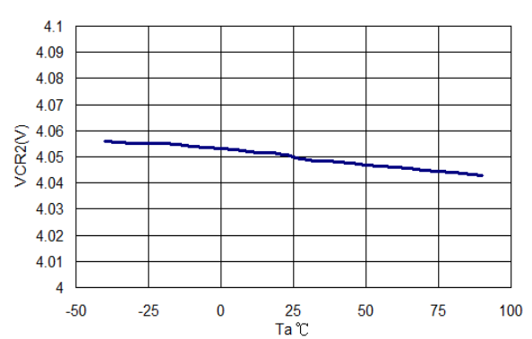
(6) V_{CR2} vs. T_a
