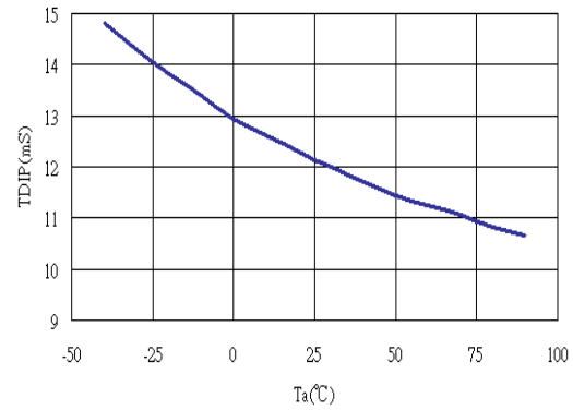
(8) T_{DIP} vs. T_a
