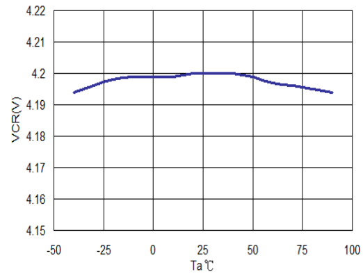
(2) V_{CR} vs. T_a
